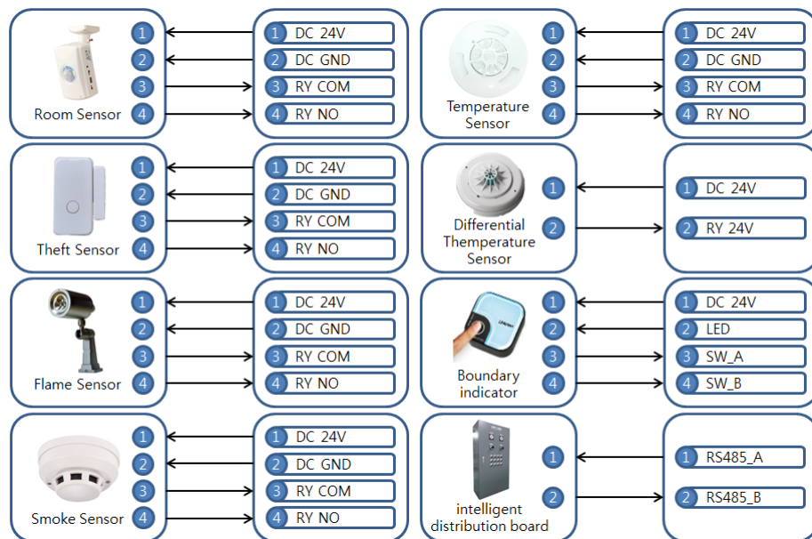
Fig. 5 Sensor Interface Circuit
